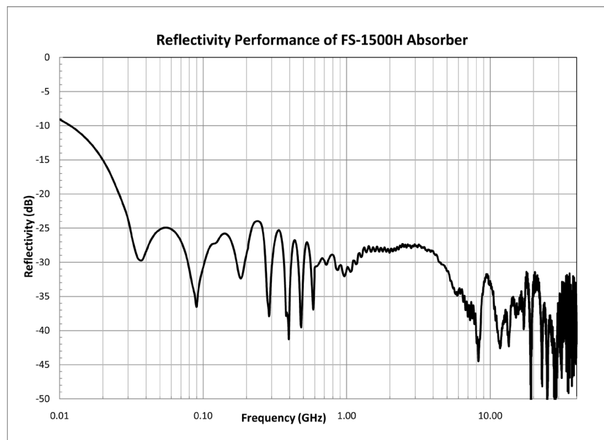
FS-1500H Typical Measured Performance
