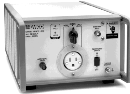
Model 3816/2 Front View
