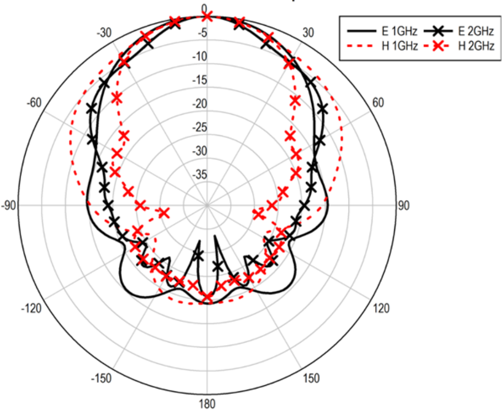
3119 Measured Patterns E and H plane
