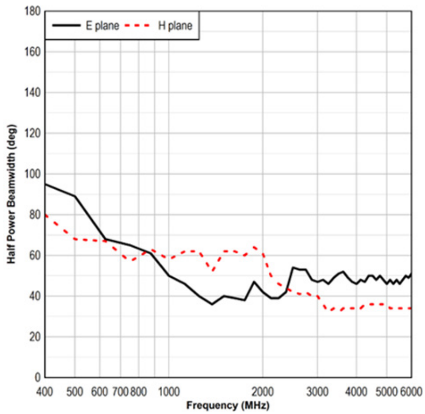
3119 Half Power Beamwidth
