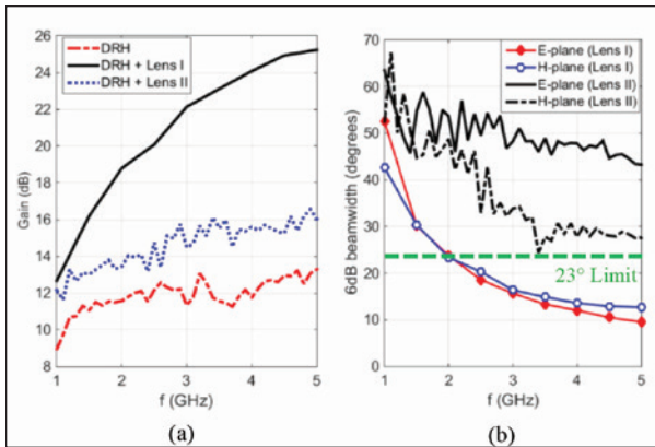
Figure 18: Simulated results of a typical DRH with lenses, (a) gain, (b) 6 dB beamwidth [11]
