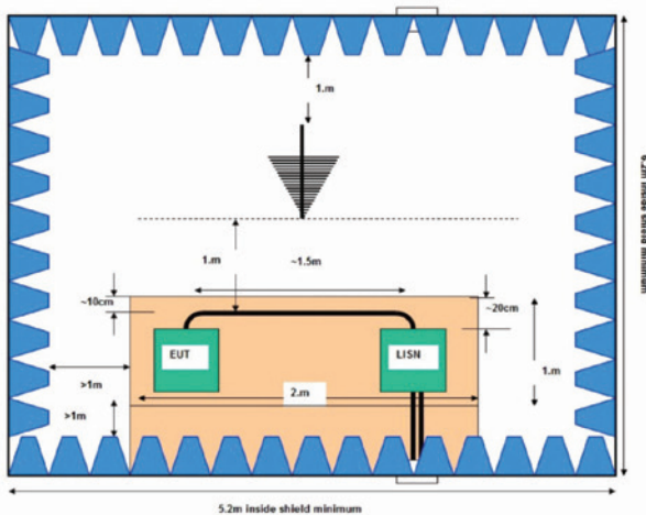
Figure 7: Determining the length of the chamber for CISPR 25
